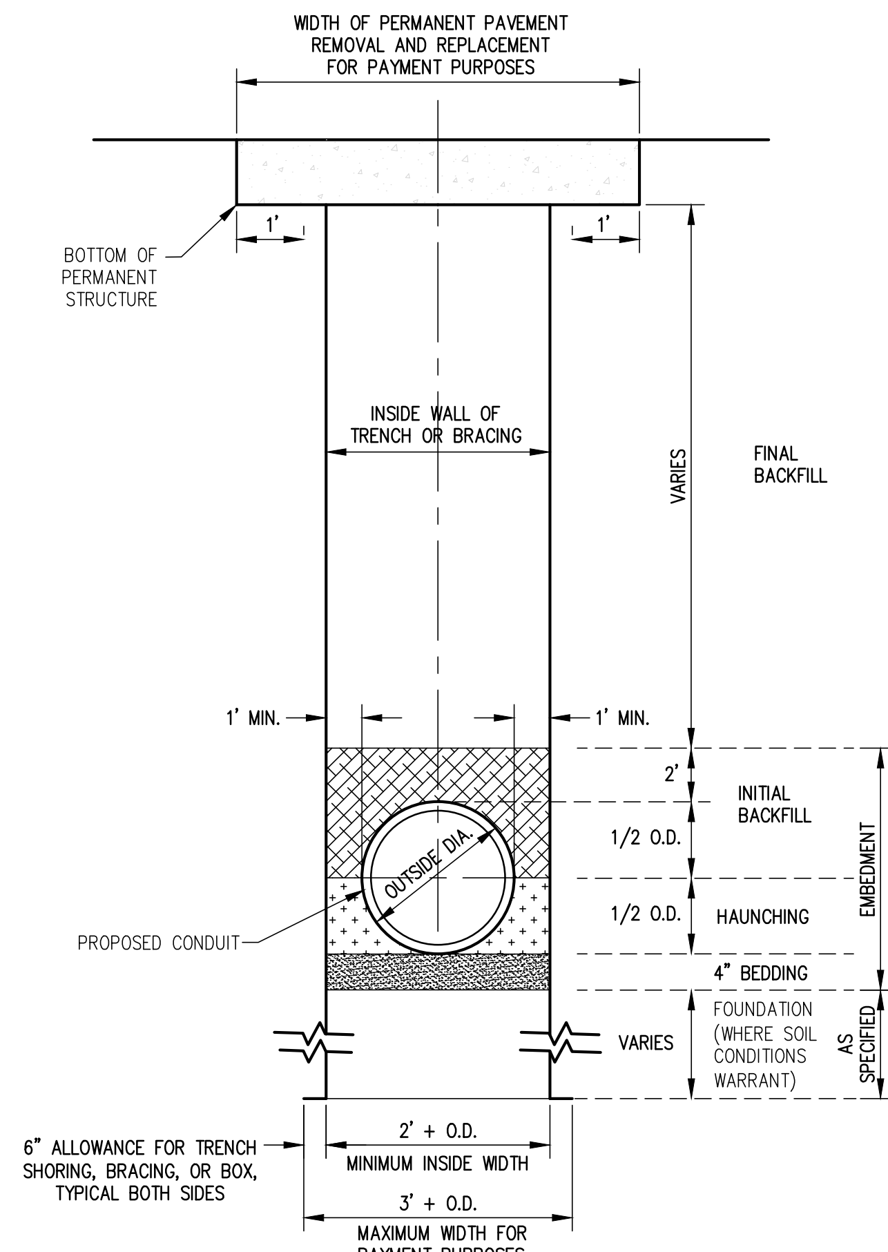
TYPICAL TRENCH DETAIL SCALE: NONE
