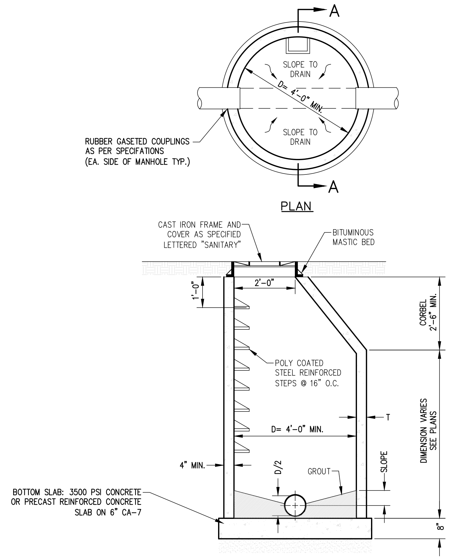
TYPICAL MANHOLE DETAIL SCALE: NONE
